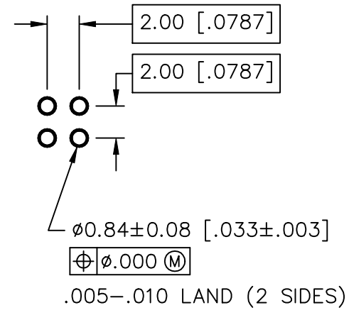
3 RECOMMENDED PRINTED CIRCUIT BOARD HOLE CONFIGURATION
