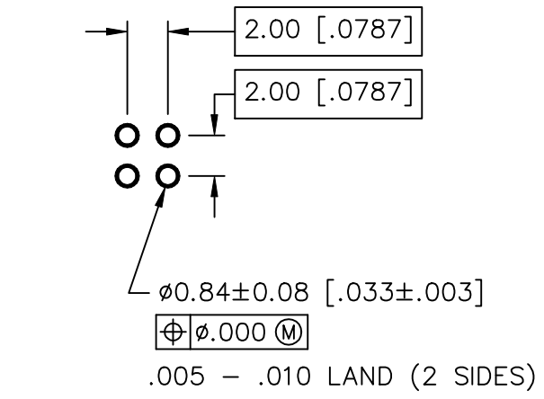
3 RECOMMENDED PRINTED CIRCUIT BOARD HOLE CONFIGURATION
